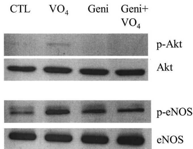
Fig. 5. Vanadate (VO 4 )-induced Akt and eNOS phosphorylation is tyrosine kinase-dependent. BLMVEC were pretreated with vehicle (EtOH) or genistein (Geni; 50 μM) for 30 min and then incubated with sodium vanadate (1 mM) for 45 min. After cell lysis, samples were subjected to SDS-PAGE and membranes were blotted with a phospho-specific anti-Akt or anti-eNOS Ser-1179 Abs, stripped, and reblotted with anti-total Akt or eNOS Abs.
